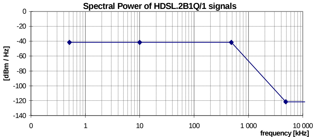
Figure 16: Spectral Power, for HDSL.2B1Q/1 signals, as specified in table 22
