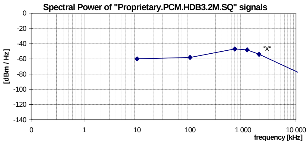
Figure 38: Spectral Power, for Proprietary.PCM.HDB3.2M.SQ signals, as specified in table 65
